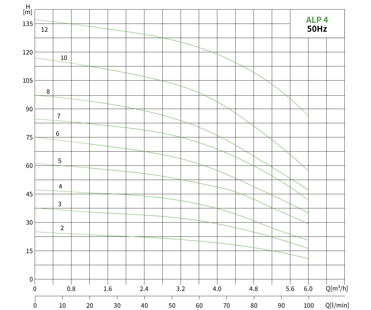
性能曲线图 Performance Curves
