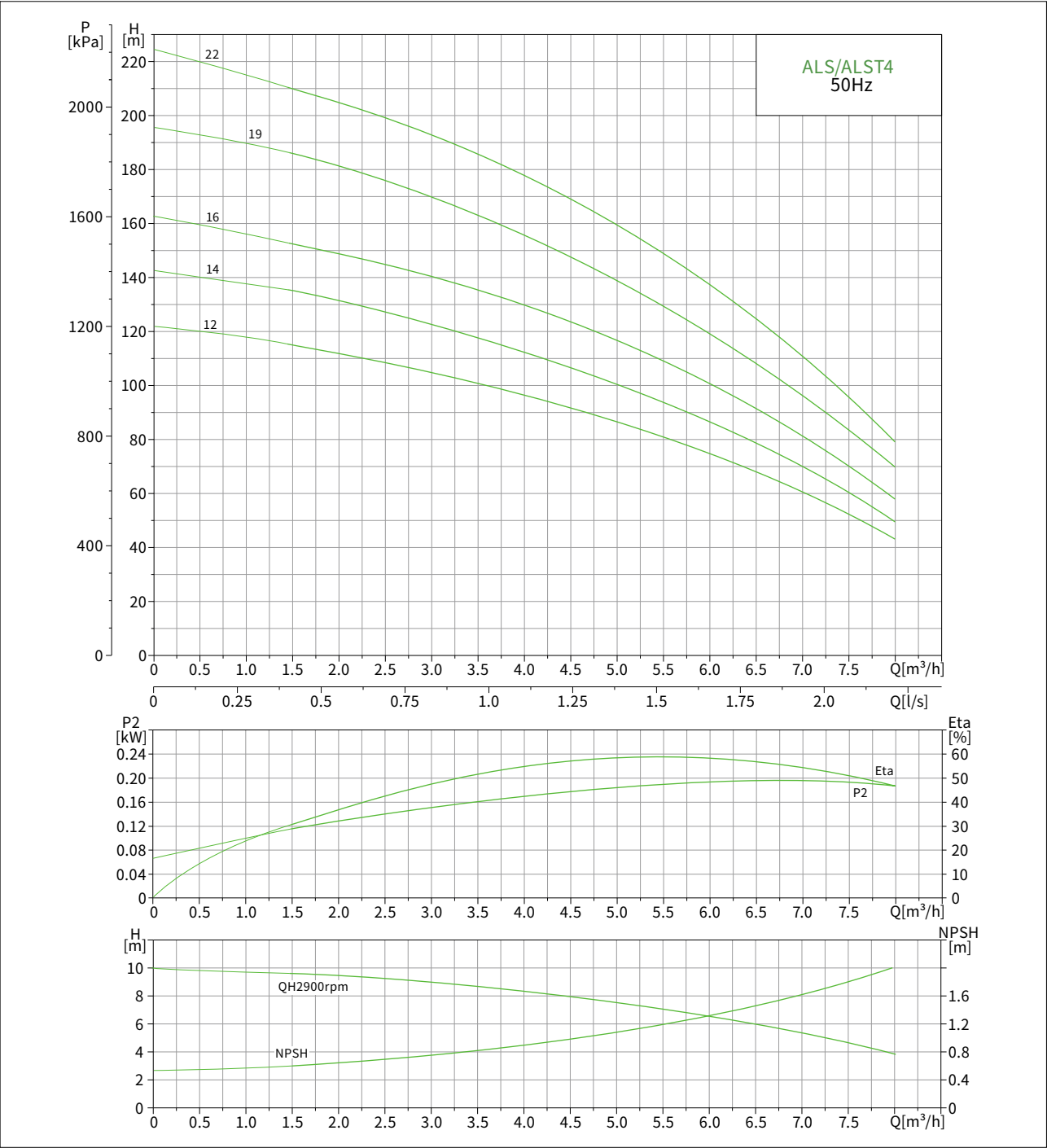
性能曲线图 Performance Curves
