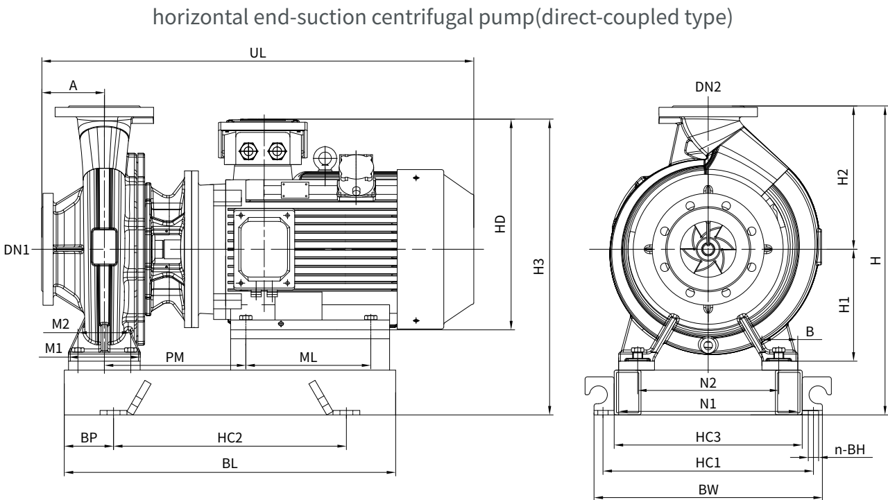
4-pole motor
