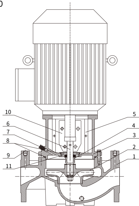
Sectional view ALG32~ALG150
